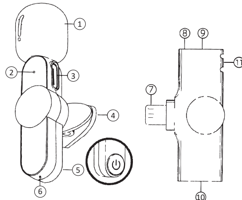
fig.1: Transmitter
